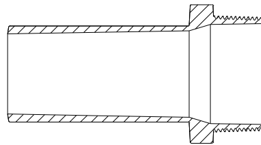
SECTION J-J
