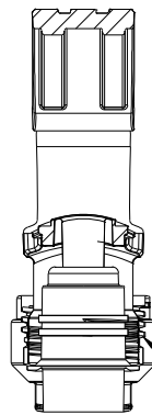
SECTION H-H
