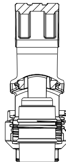
SECTION F-F
