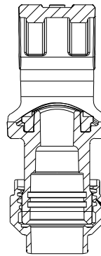
SECTION C-C
