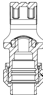
SECTION B-B
