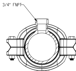
SECTION F-F
