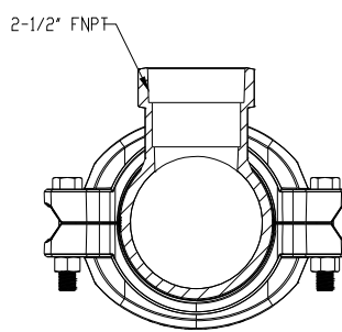
SECTION E-E
