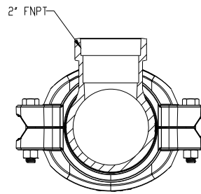
SECTION I-I
