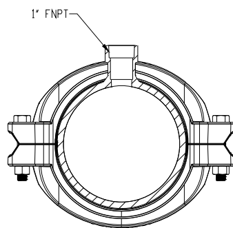
SECTION G-G
