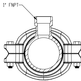
SECTION G-G
