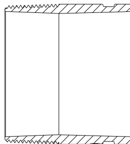
SECTION K-K
